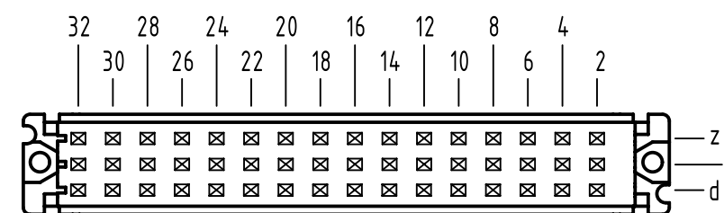
contact arrangement
