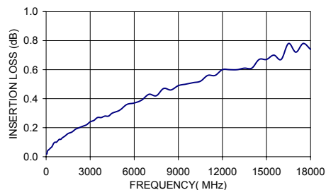
141-12SM+ INSERTION LOSS
