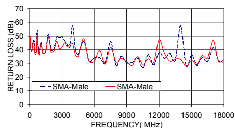
141-12SM+ RETURN LOSS
