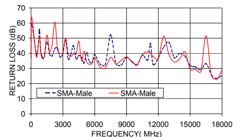
141-6SM+ RETURN LOSS
