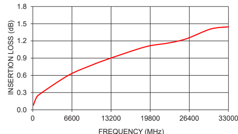
FL86-12SSMPSMP+ INSERTION LOSS
