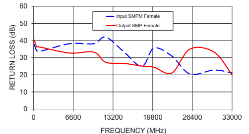
FL86-12SSMPSMP+ RETURN LOSS
