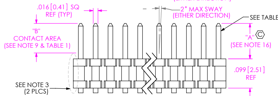
FIG 1 FTSH-1XX-XX-XXX-DV SHOWN
