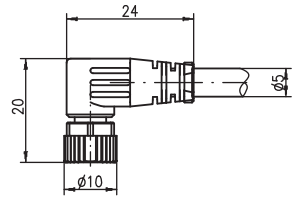
M8 cable angular socket, 3/4-pin K-D M8W-...-PUR
