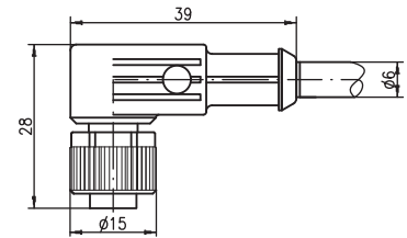
M12 cable angular socket, 4/5-pin K-D M12W-...-DP-PUR (LEDs)
