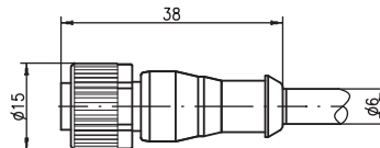
M12 cable axial socket, 4-pin K-D M12A-...-DP-PUR (LEDs)
