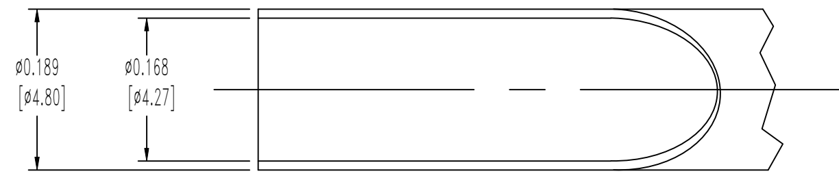
DETAIL A
