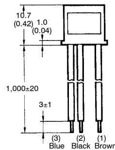
Terminal Arrangement
