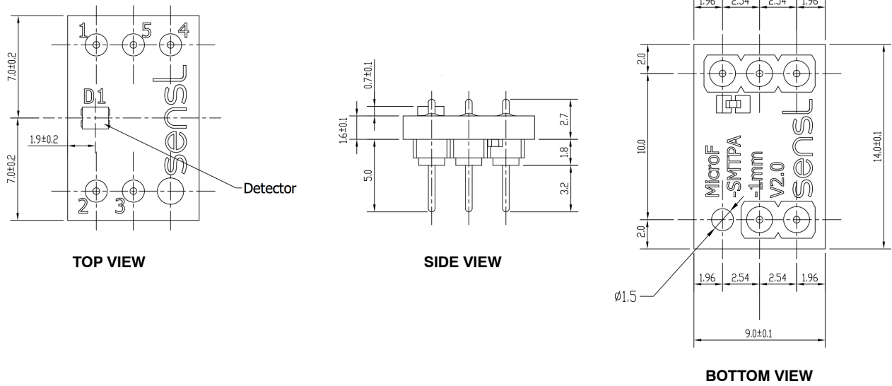
MICRORB-SMTPA-100XX
