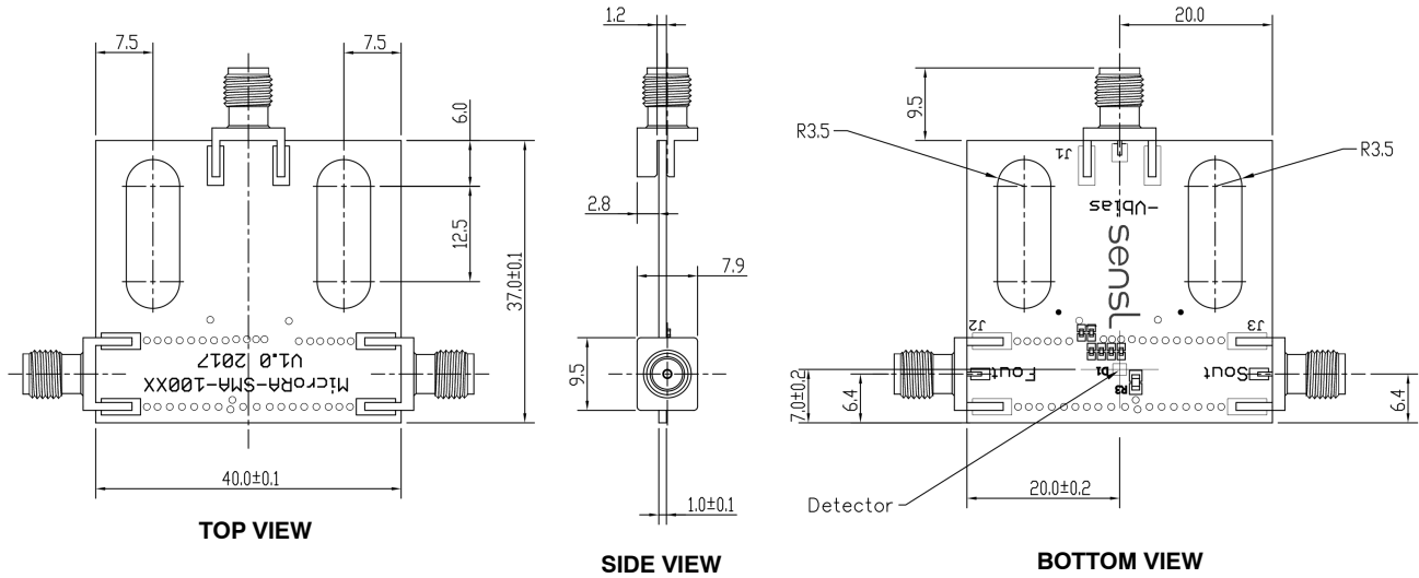
MICROB-SMA-100XX
