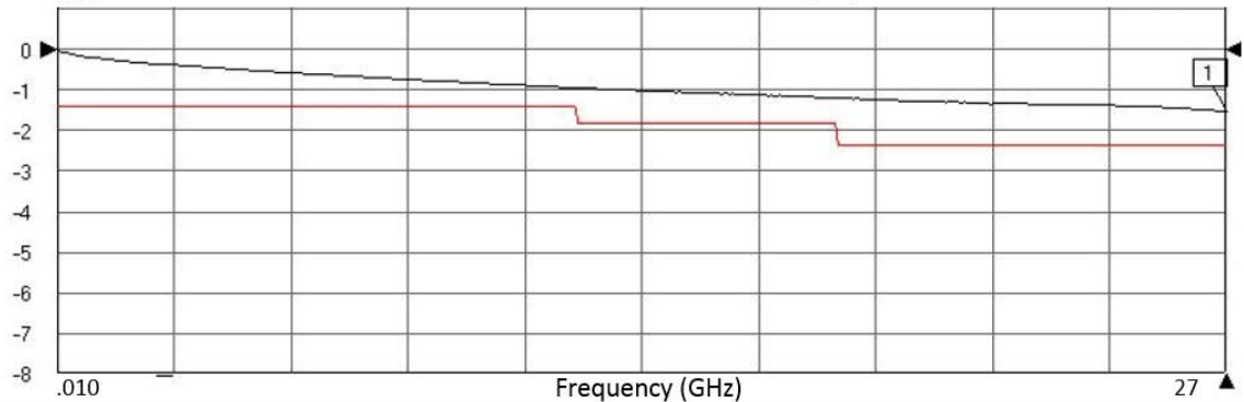
S12 PE3TC0201-24 Insertion Loss (dB)
