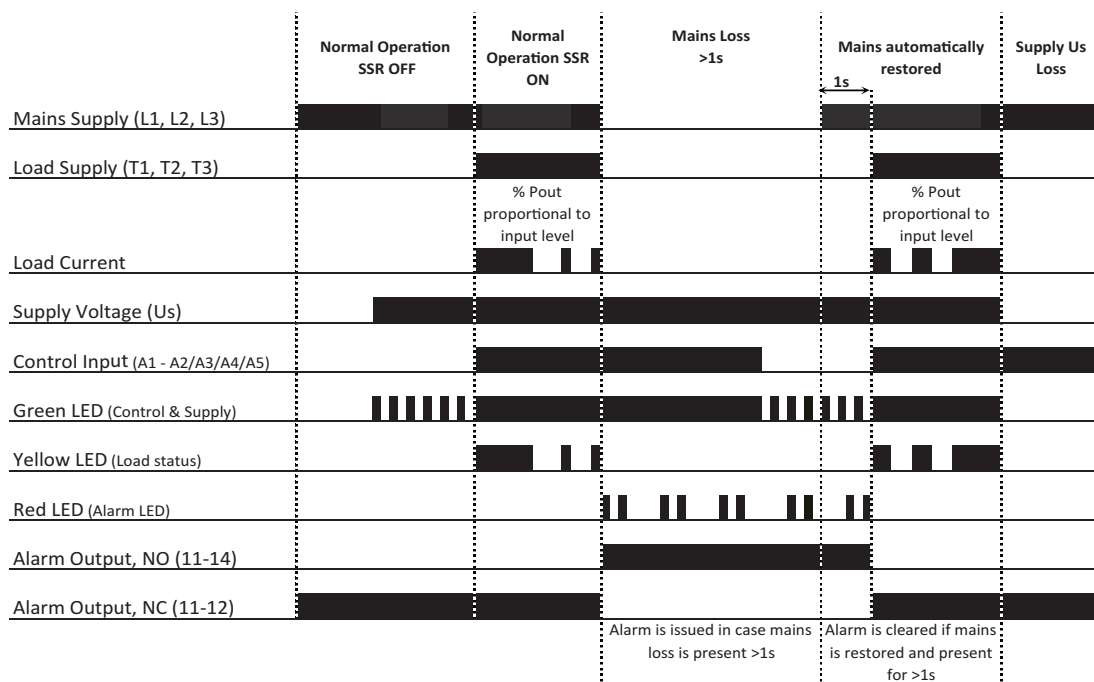
Operation Diagram 3:
