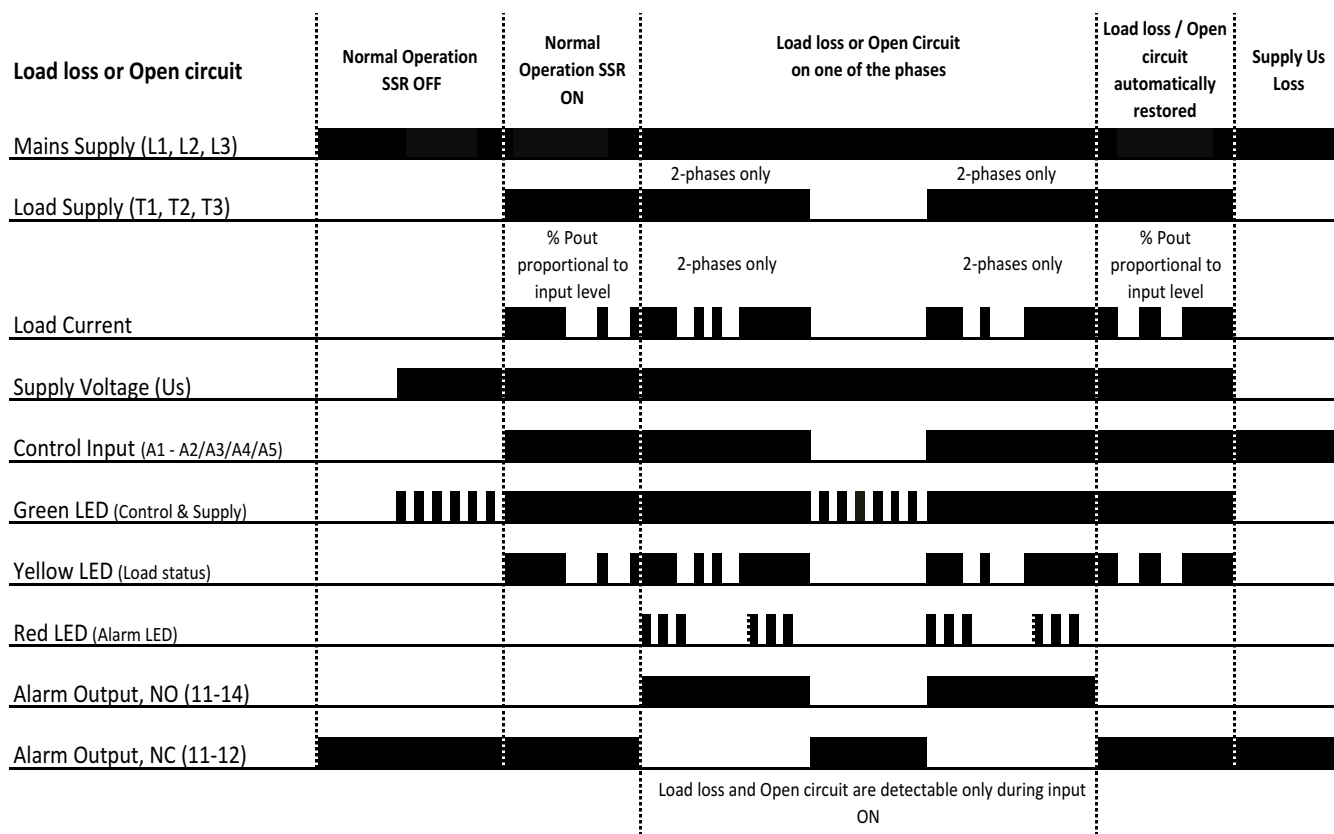
Operation Diagram 4:
