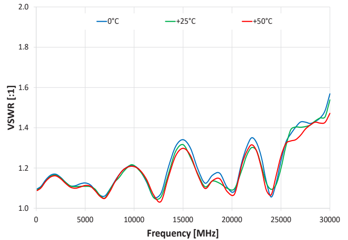
VSWR @ J2 over Temperature (J2 Terminated)
