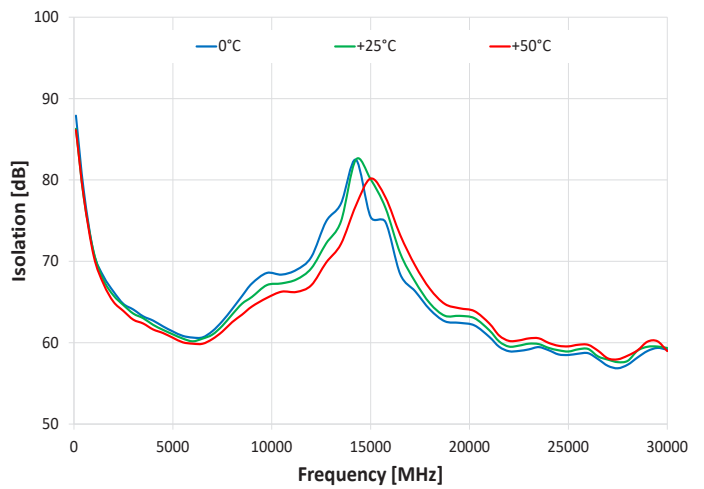
Isolation J1 to J2 (J2 Active)
