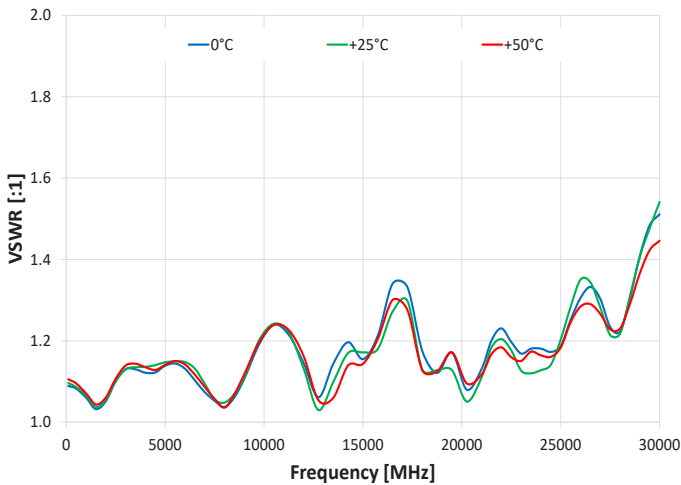
VSWR @ J2 over Temperature (J2 Active)
