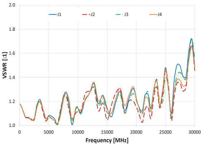
VSWR @ Active ports (J1- J4 Active)
