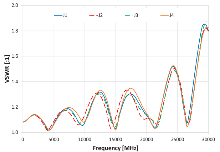
VSWR @ Terminated ports (J1 - J4 Terminated)
