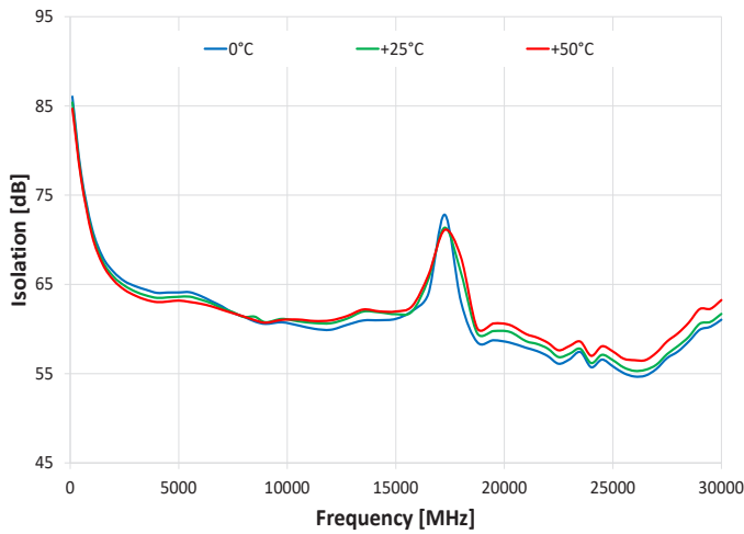
Isolation J2 to J3 (J3 Active)
