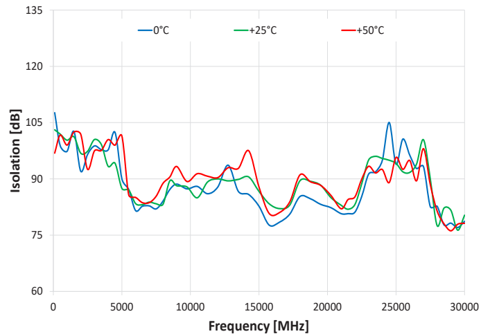
Isolation J4 to J5 (J4 Active)
