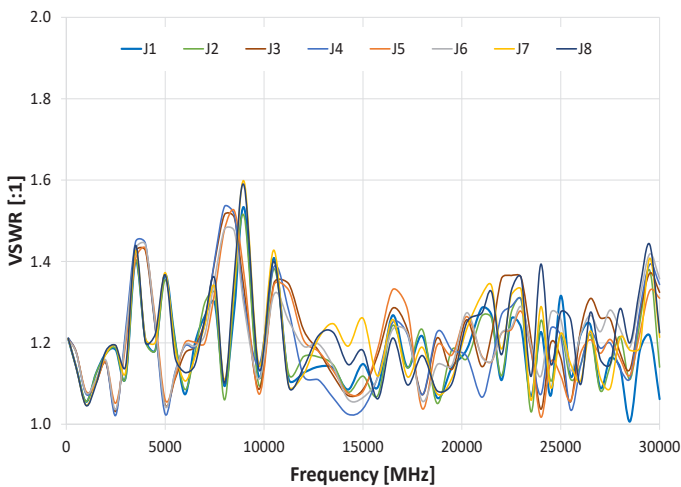
VSWR @ Active ports (J1- J8 Active)
