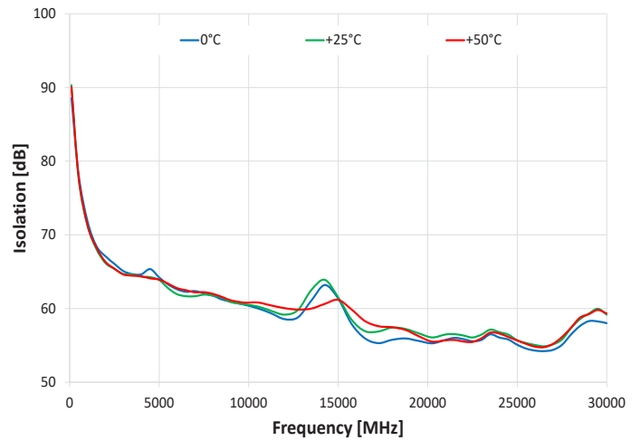
Isolation J4 to J5 (J4 Active)
