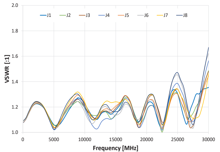
VSWR @ Terminated ports (J1 - J8 Terminated)
