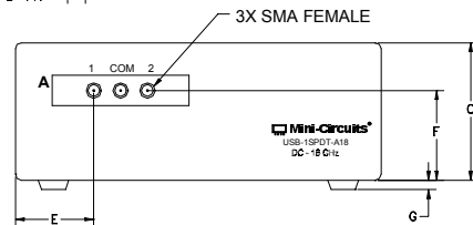
FRONT VIEW (SCALE 1.5:1)
