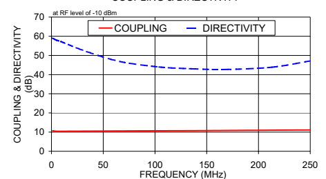
ZDC-10-1-75+ COUPLING & DIRECTIVITY
