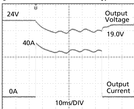
Fig. 26-3 Peak load 40A for 50ms, typ.
