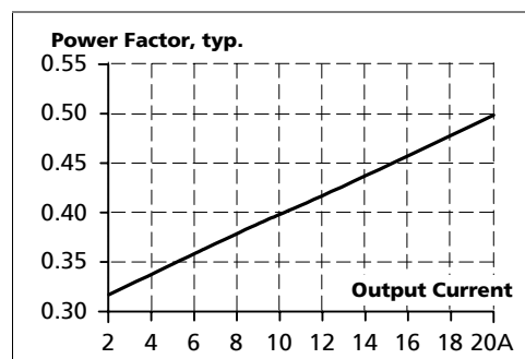
Fig. 5-4 Power factor vs. output load at 230Vac
