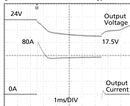
Fig. 26-4 Peak load 80A for 5ms, typ.
