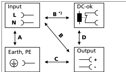
Fig. 18-1 Dielectric strength
