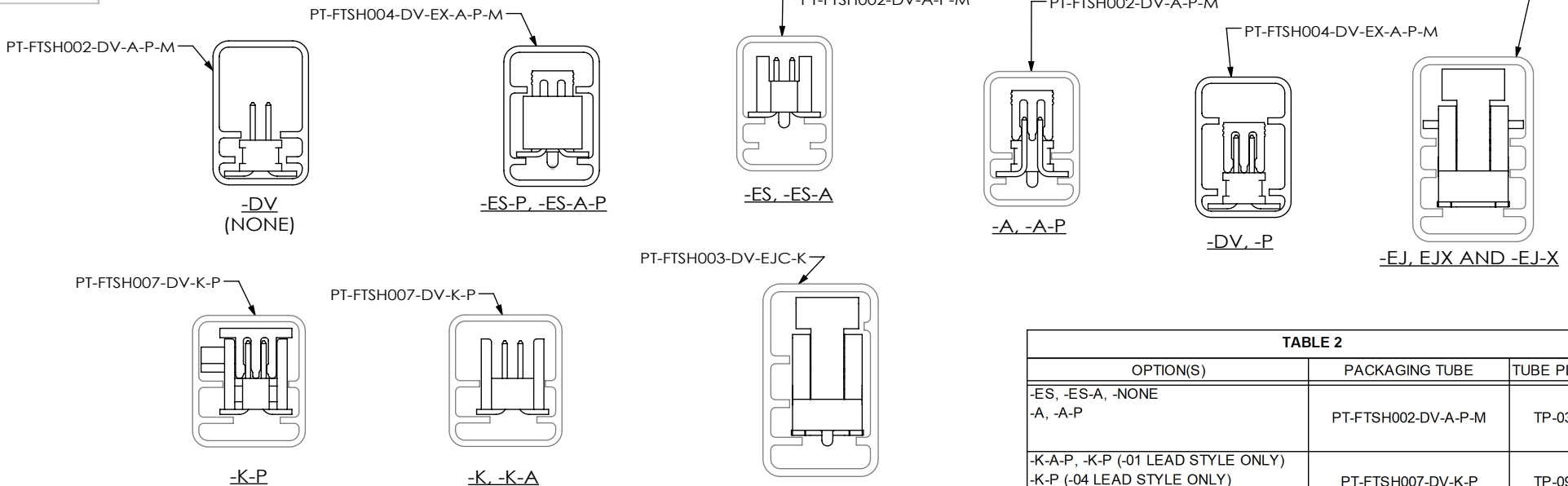
FIG 13 TUBE VIEWS
