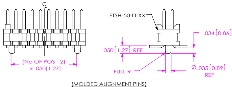
FIG 3 -A OPTION (DIFFERENT AS SHOWN, OTHERWISE SAME AS FIG 1) (6 POSITION MINIMUM FOR STAKED ALIGNMENT PINS) (3 POSITION MINIMUM FOR MOLDED ALIGNMENT PINS)
