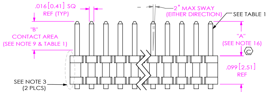
FIG 1 FTSH-1XX-XX-XXX-DV SHOWN
